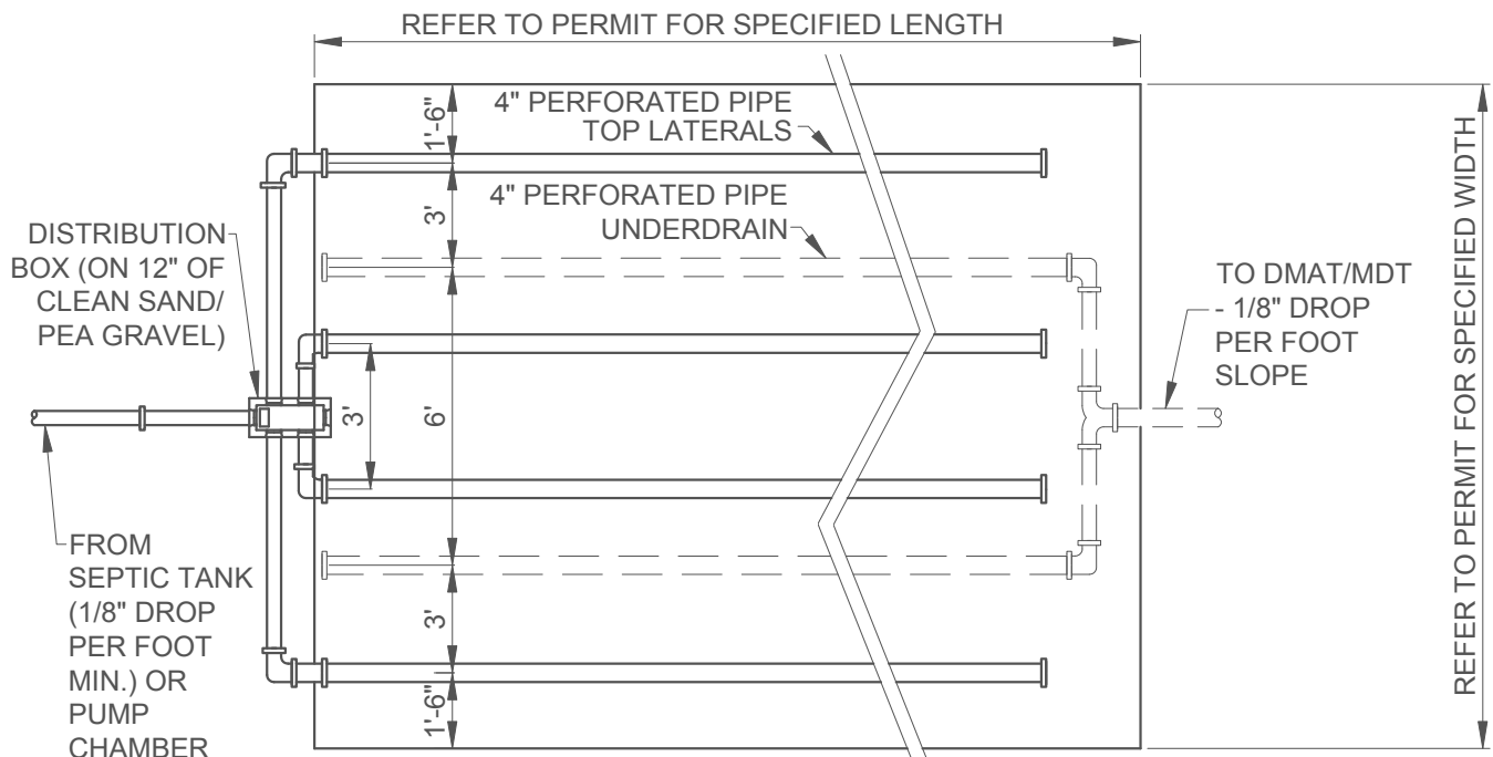
TOP VIEW - NOT TO SCALE
